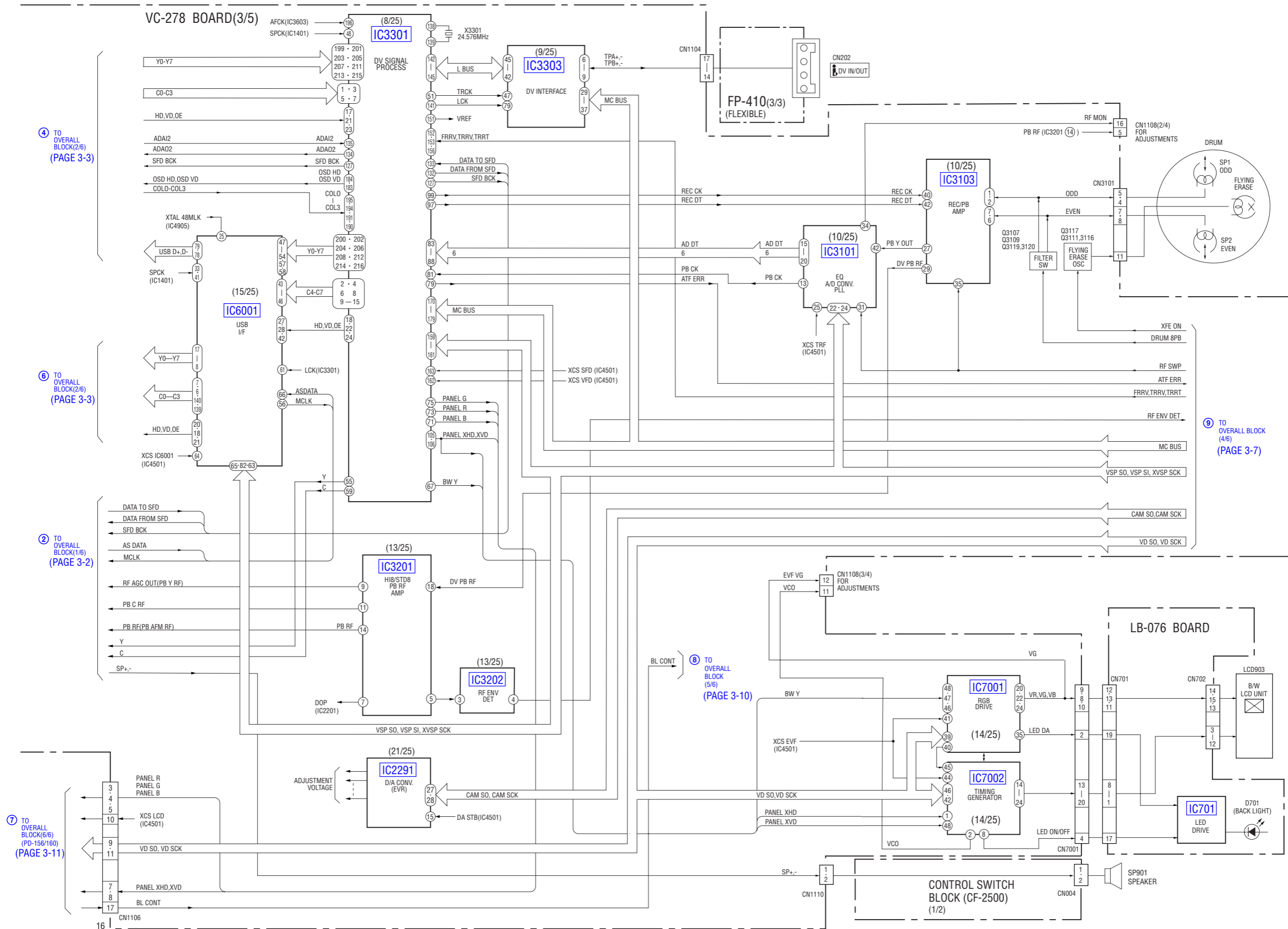
3-3. OVERALL BLOCK DIAGRAM (3/6) ( ) : Number in parenthesis ( ) indicates the division number of schematic diagram where the component is located.
